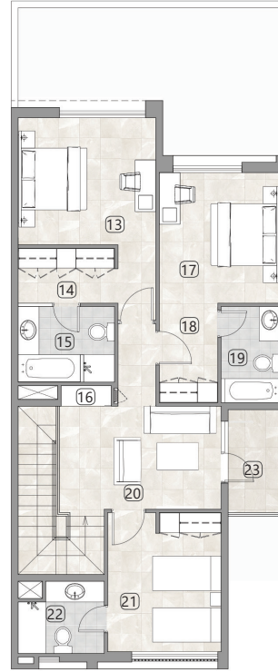
FIRST LEVEL PLAN
