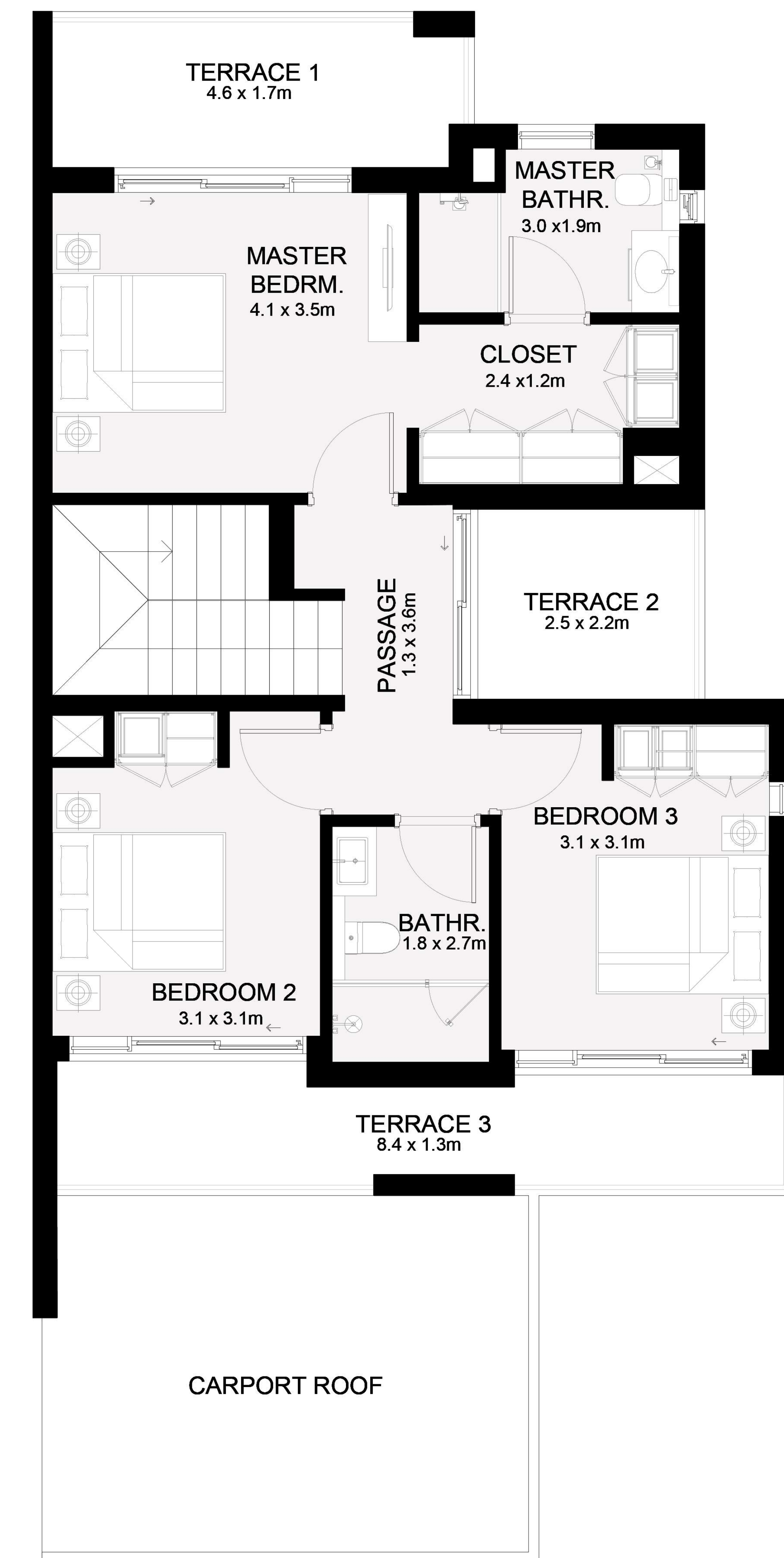
FIRST FLOOR
