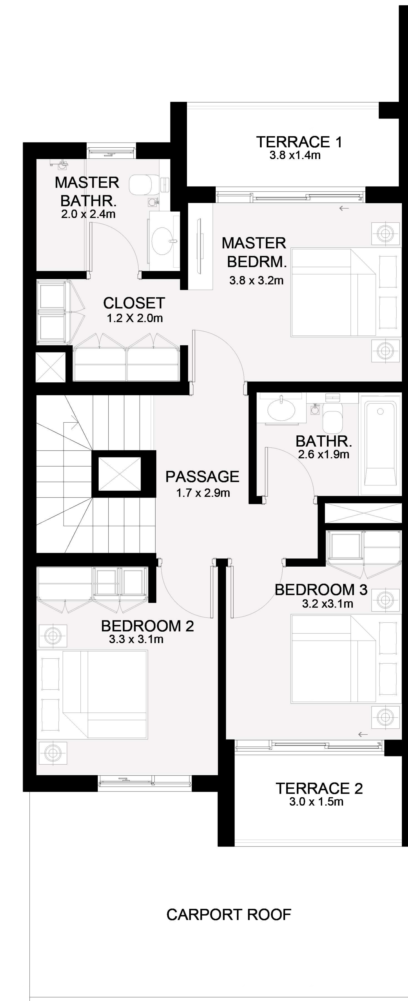
FIRST FLOOR
