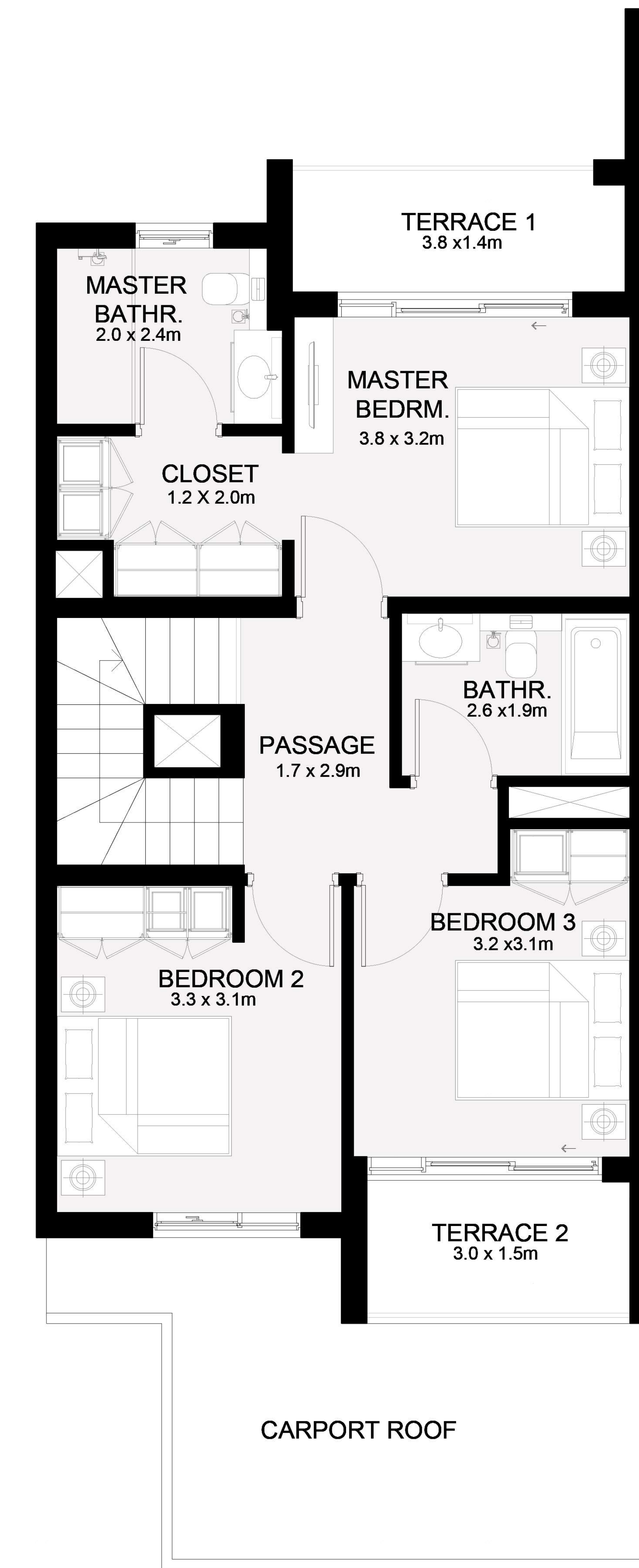
FIRST FLOOR
